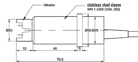
Type 3205.30: Techn. Data as 3202.30 max. pressure 10 bar, installation with union nut G 1" A, SW 37 mm, DIN 259, ISO 228 mass approx. 200 g without nut
