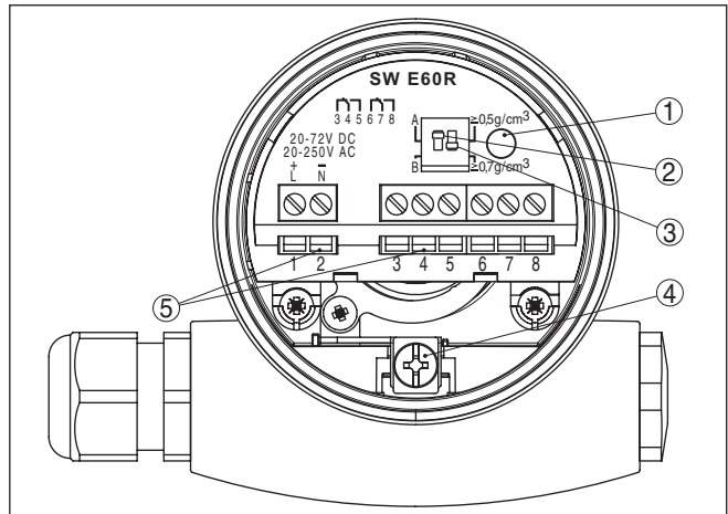
Fig. 10: Electronics and terminal compartment, single chamber housing
