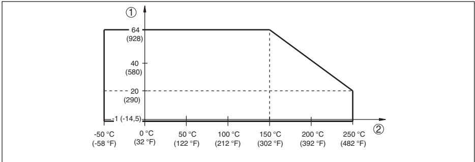
Fig. 34: Process temperature - Process pressure with switch position \geq 0.5 \text{ g/cm}^3 (sensitivity switch)
