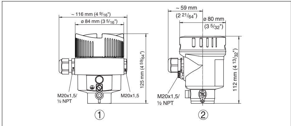
Fig. 35: Housing versions
