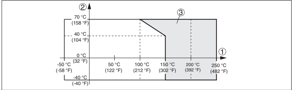
Fig. 32: Ambient temperature - Process temperature
