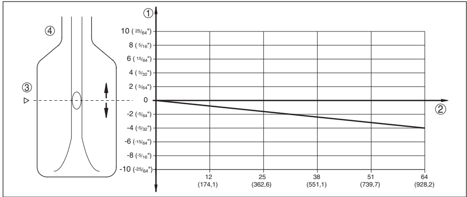
Fig. 31: Influence of the process pressure to the switching point
