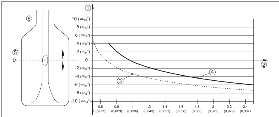
Fig. 30: Influence of the product density on the switching point
