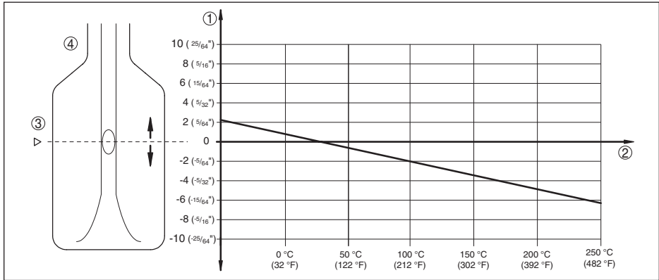
Fig. 29: Influence of the process temperature on the switching point
