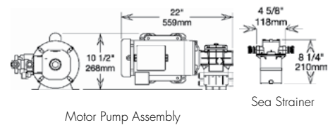
Motor Pump Assembly
