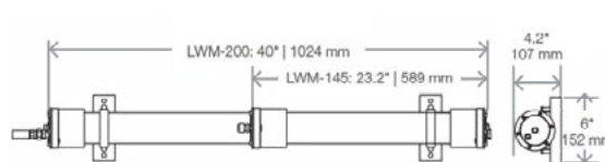
Membrane Assembly
