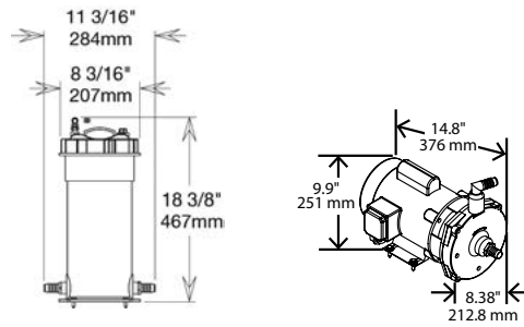
Commercial Pre-Filter & Oil Water Separator
