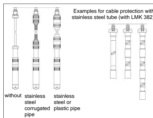
Fig. 3: Cable protection variants
