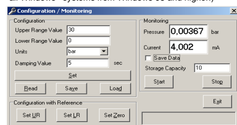
Fig. 4 Configuration software
