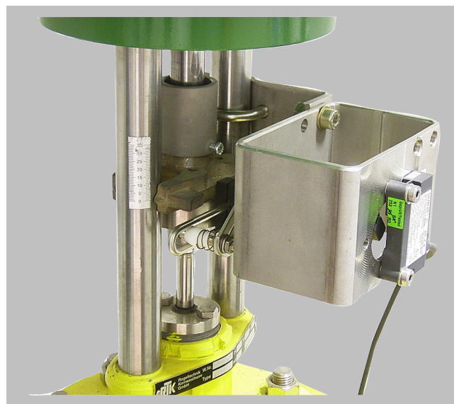
SIPART PS2, NCS for strokes > 14 mm
