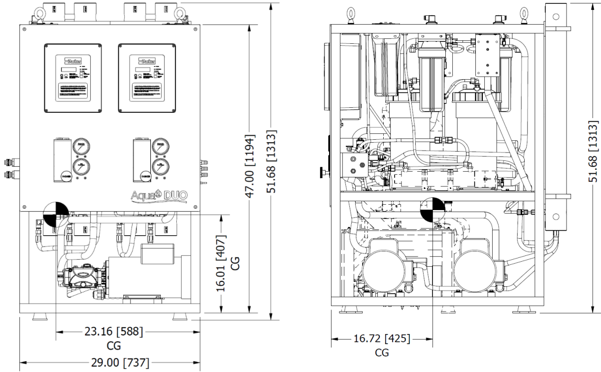
Figure 1.0: 2800-3600 GPD RO System Dimensions
