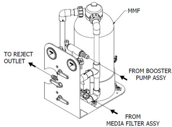
Figure 2.12: Optional Media Filter Assembly (MMF-1 & MMF-2)
