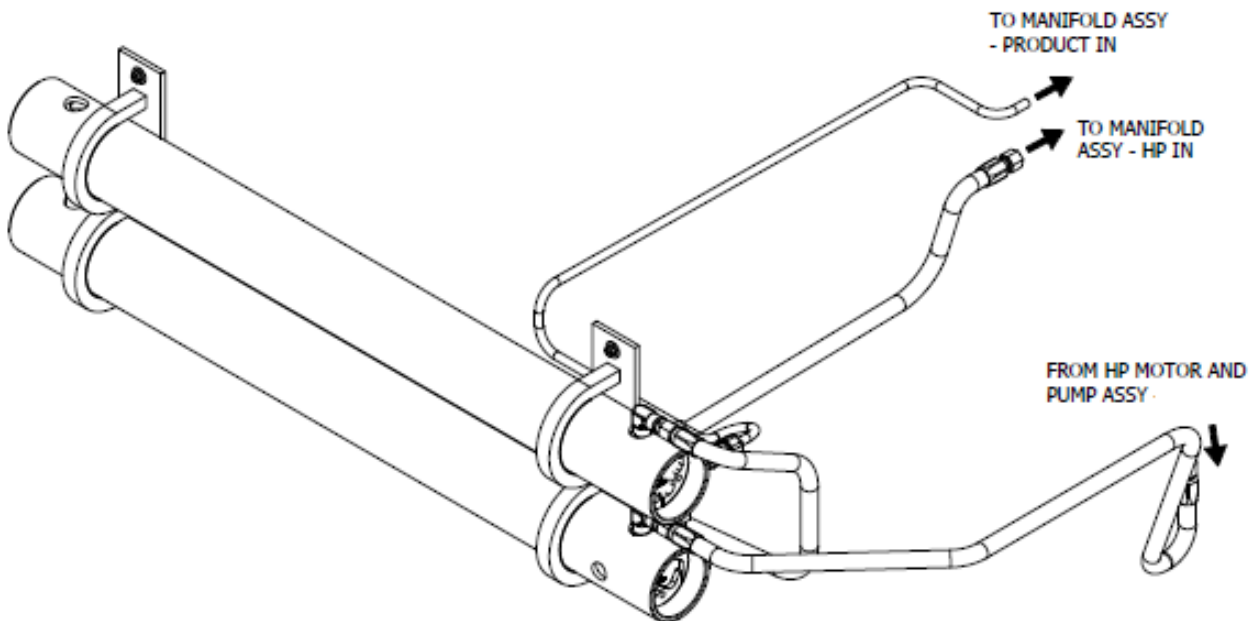
Figure 2.24: Two Vessel Assembly
