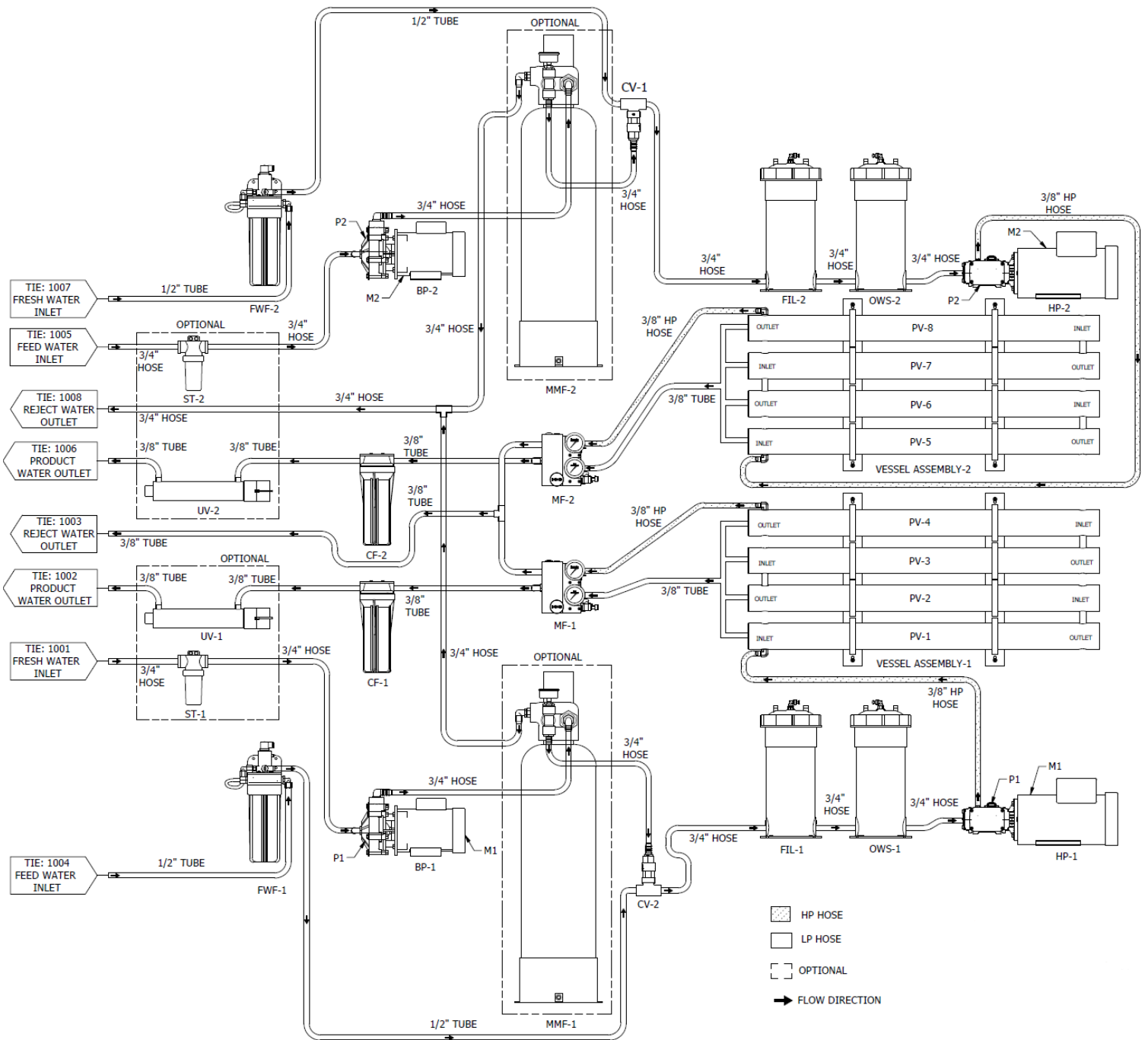
Figure 2.6: Piping and Instrumentation Diagram 4800-6200 GPD
