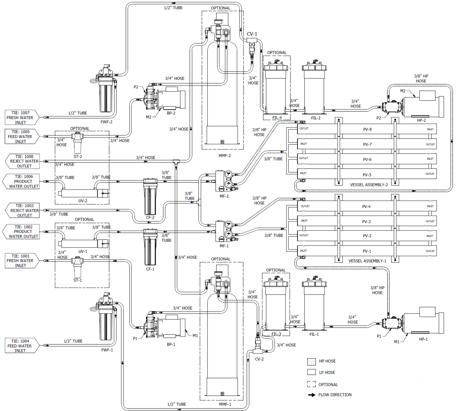
Figure 2.7: Piping and Instrumentation Diagram 4800-6200 GPD (with Optional 20-Micron Prefilter)
