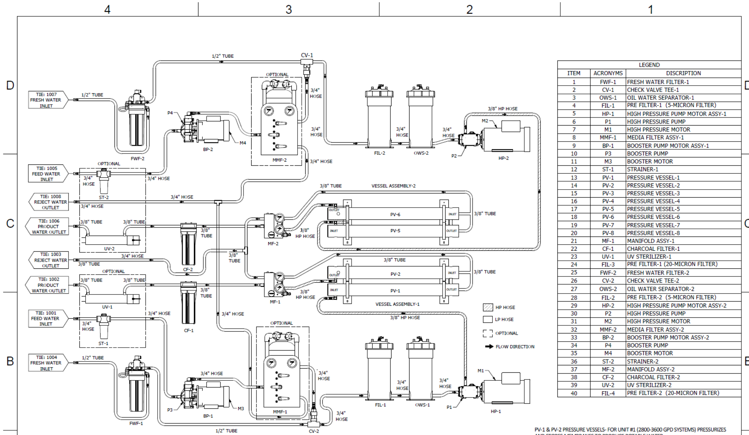
PLUMBING DIAGRAM FOR 2800-3600 GPD SYSTEM
