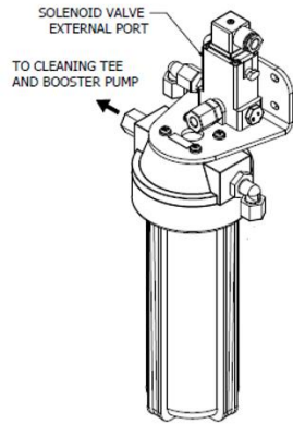
Figure 2.14: Freshwater Flush Filter (FWF-1 & FWF-2)
