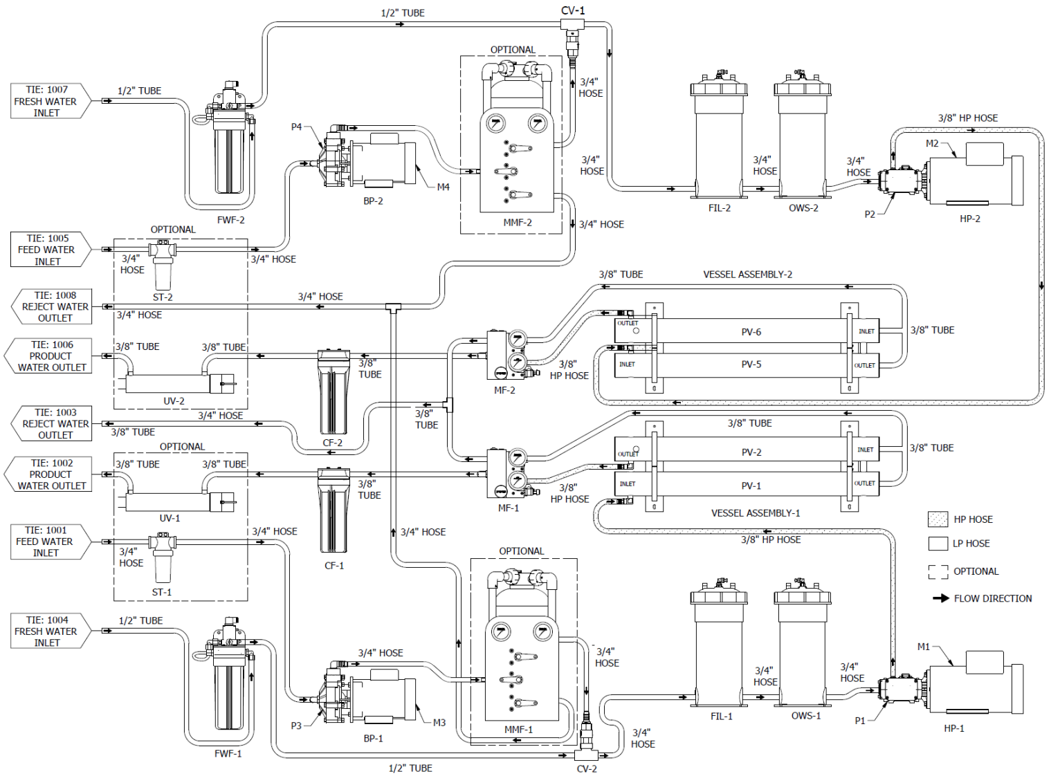
Figure 2.4: Piping and Instrumentation Diagram 2800-3600 GPD
