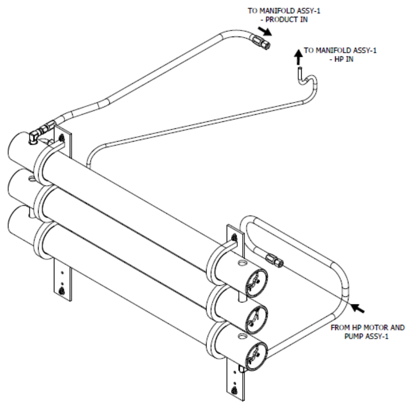
PRESSURE VESSEL ASSY-1 (LARGER)
