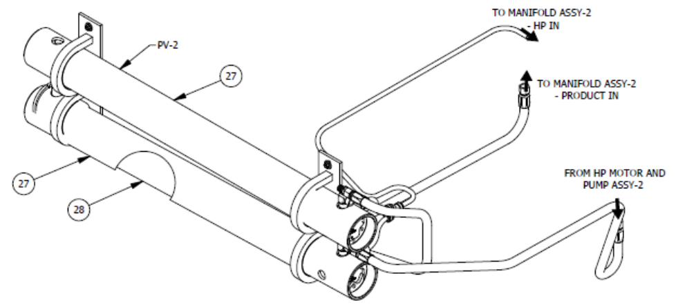
PRESSURE VESSEL ASSY-2 (SMALLER)
