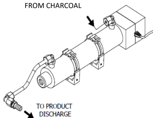
Figure 2.21: Ultraviolet Sterilizer
