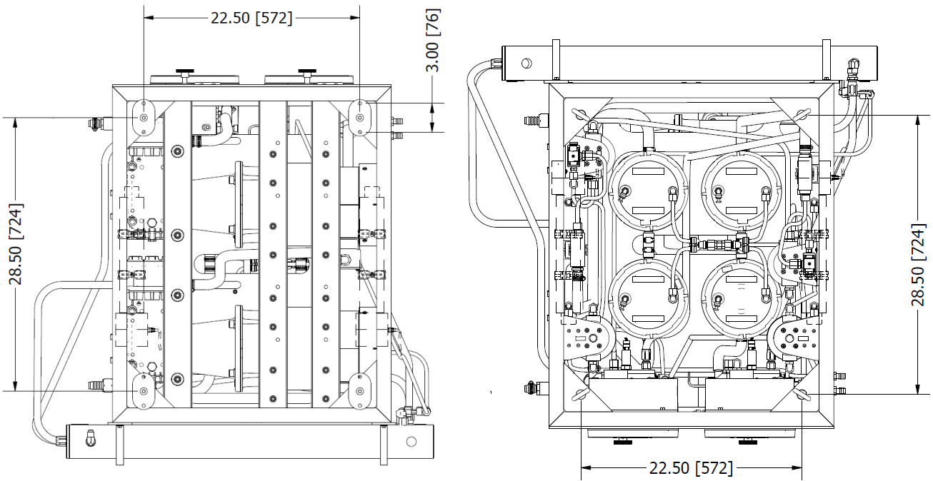
Figure 1.3: Mounting and Lifting lugs Dimensions of RO System
