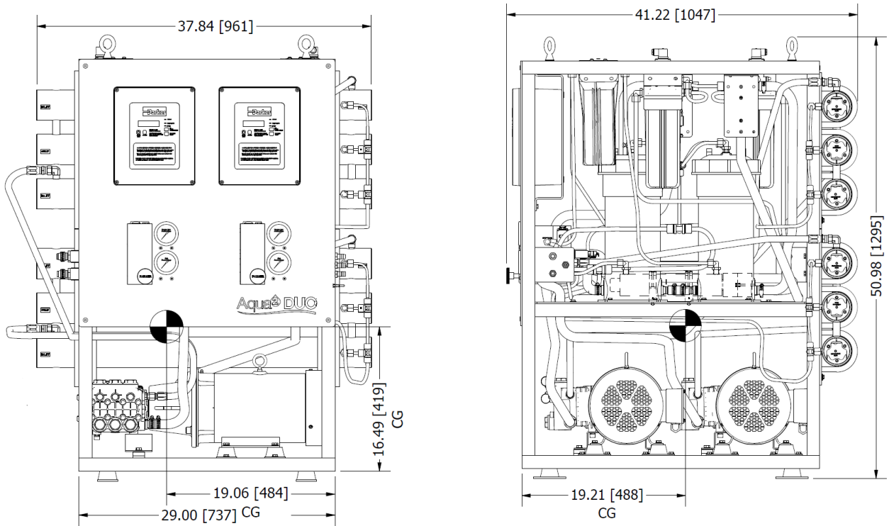
Figure 1.1: 4400 & 5800 GPD RO System Dimensions
