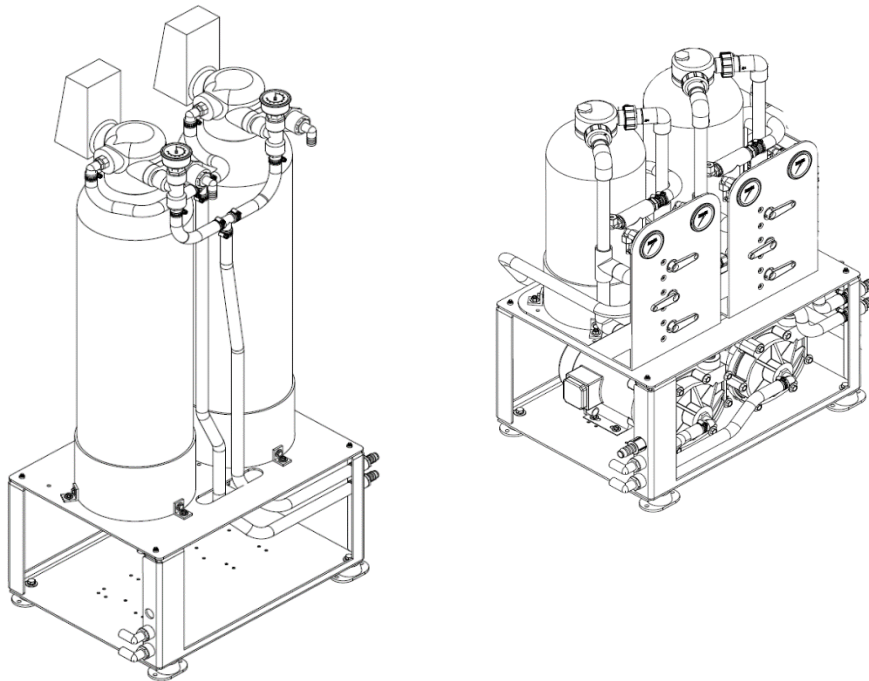
Figure 2.11: Optional Media Filter Assembly (Booster Pumps not included in KIT)
