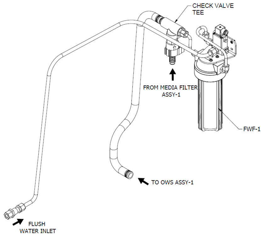
Figure 2.15: Freshwater Flush & Check Valve Assemblies
