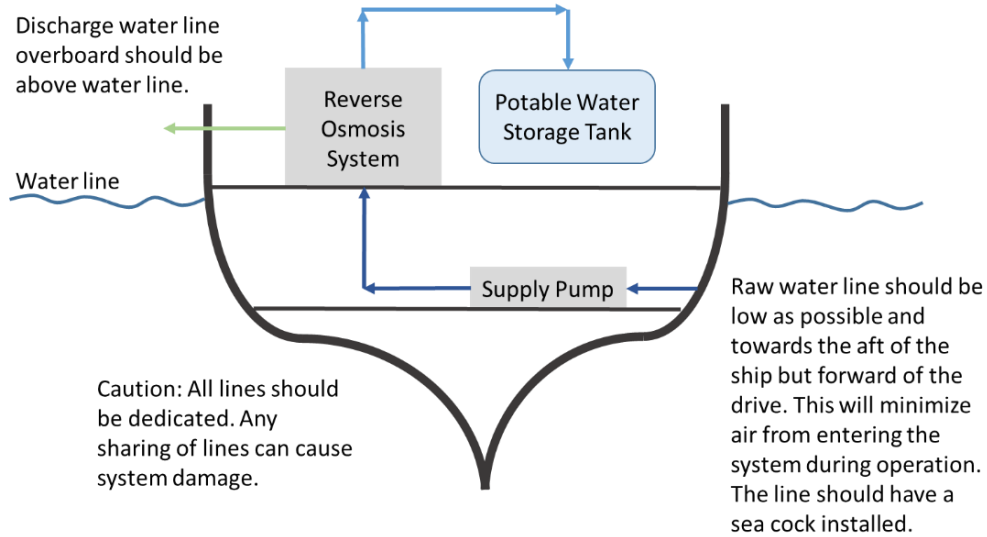
Figure 2.2: RO System Above Water Line
