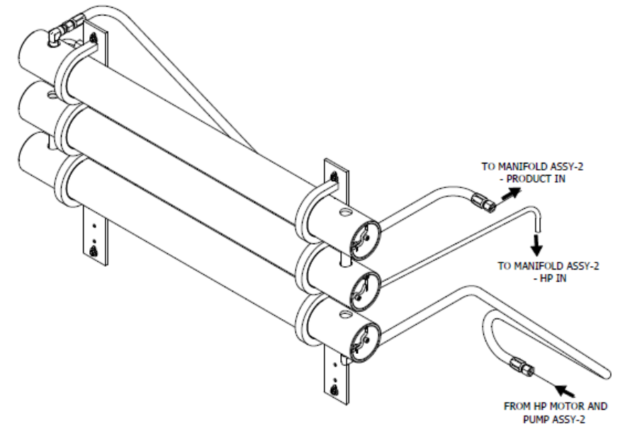
PRESSURE VESSEL ASSY-2 (LARGER)
