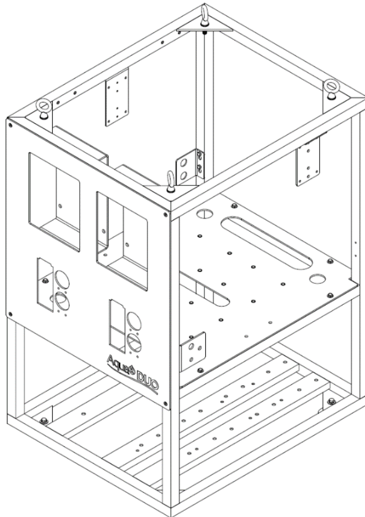
Figure 2.13: Main frame Assembly
