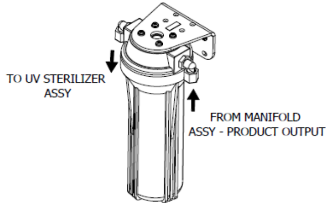
Figure 2.20 : Charcoal Filter (CF1 & CF2) assembly
