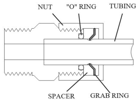
Figure 2.29: Tubing Fitting Internals
