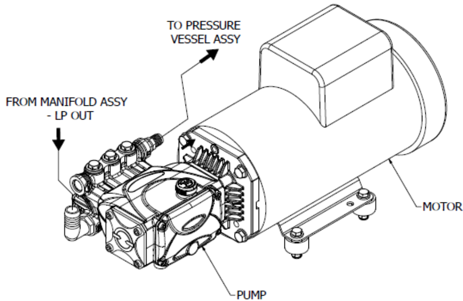
Figure 2.22: High Pressure Pump and Motor Assembly
