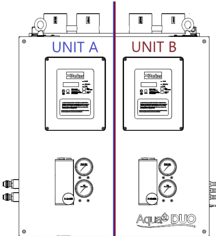
Figure 2.3: Illustration of Unit A and Unit B Controls
