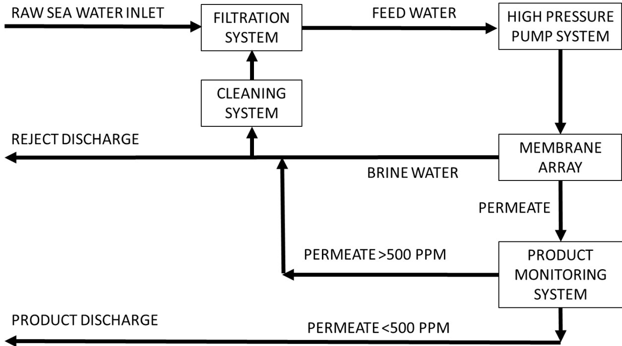
Figure 3.2: Simplified Schematic of a RO System
