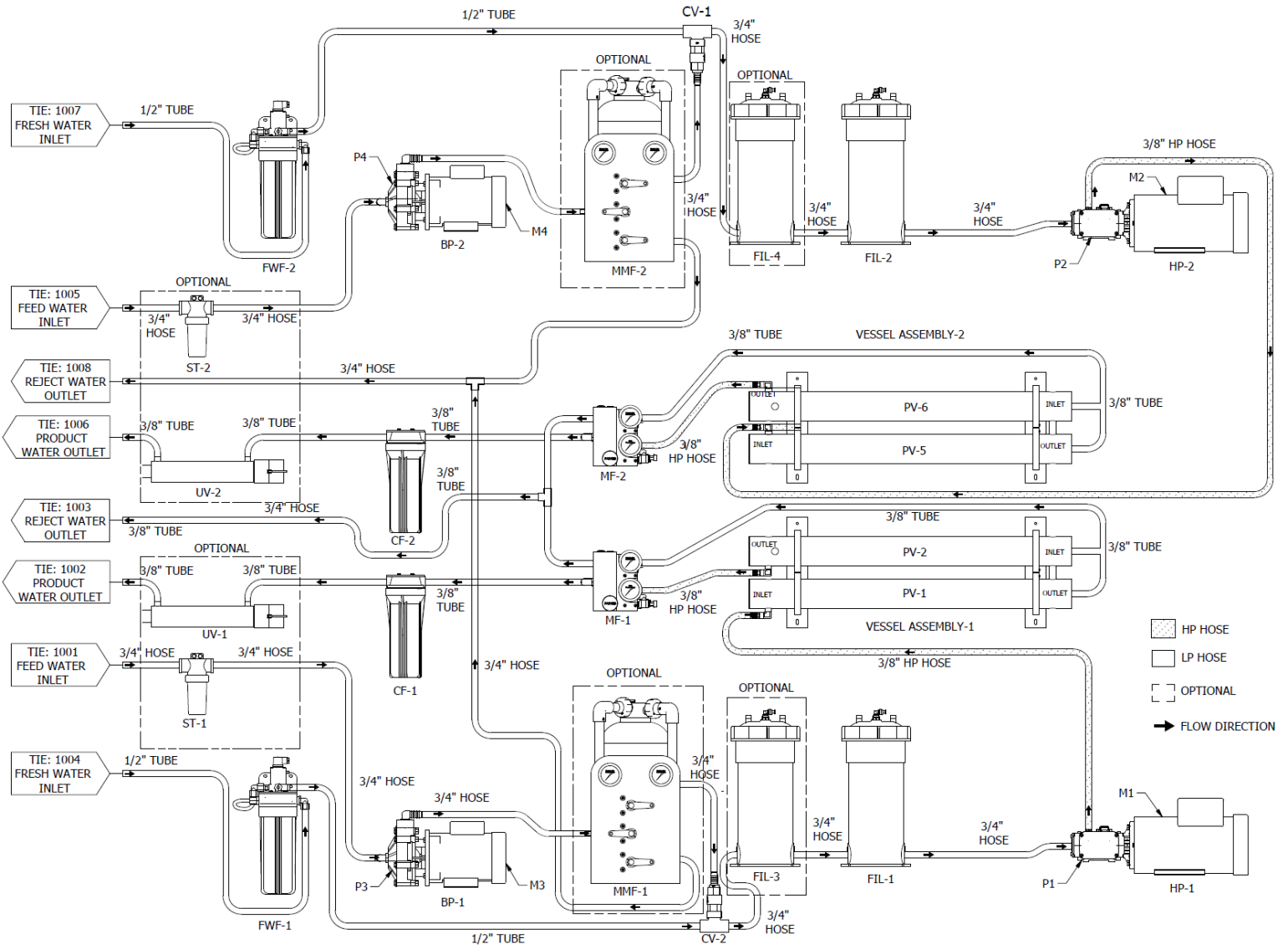
Figure 2.5: Piping and Instrumentation Diagram 2800-3600 GPD (with Optional 20-Micron Prefilter)
