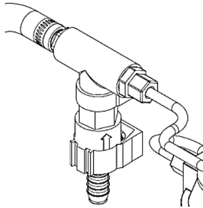
Figure 2.16: Check Valve (CV-1 & CV-2) Assembly
