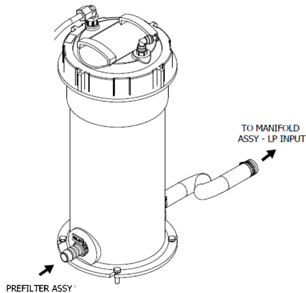
Figure 2.18: Oil & Water Separator (OWS-1 & OWS-2) Assembly
