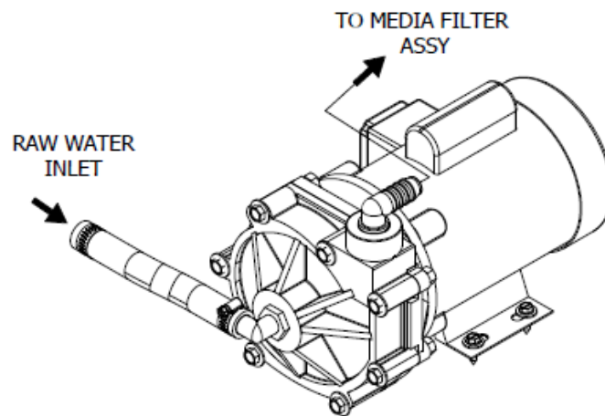
Figure 2.17: Boost Pump Assembly (BP-1 & BP-2)
