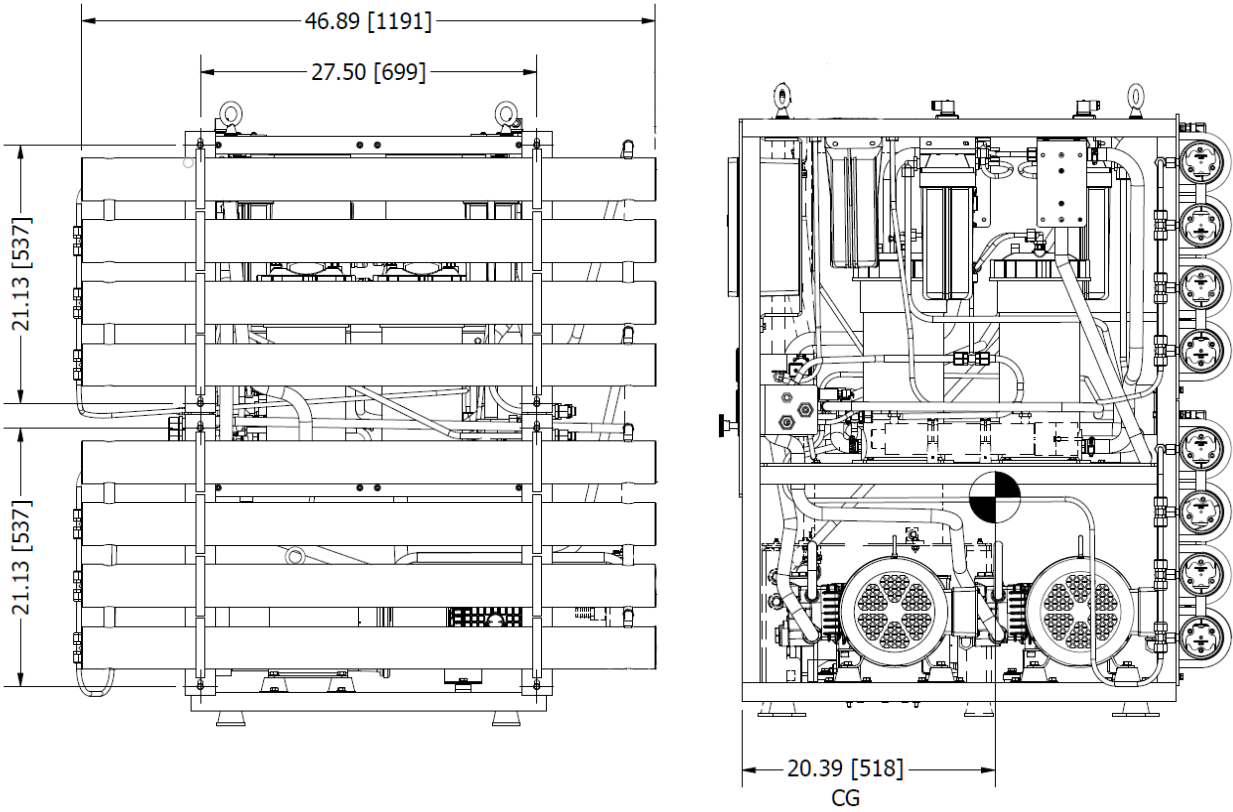
Figure 1.2: 5200 & 6800 GPD RO System Dimensions
