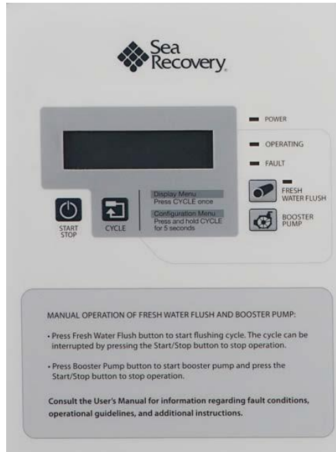
Figure 5.1: Controller Interface
