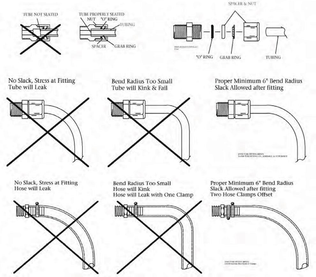
Figure 2.28: Hose & Tube Connection Instructions
