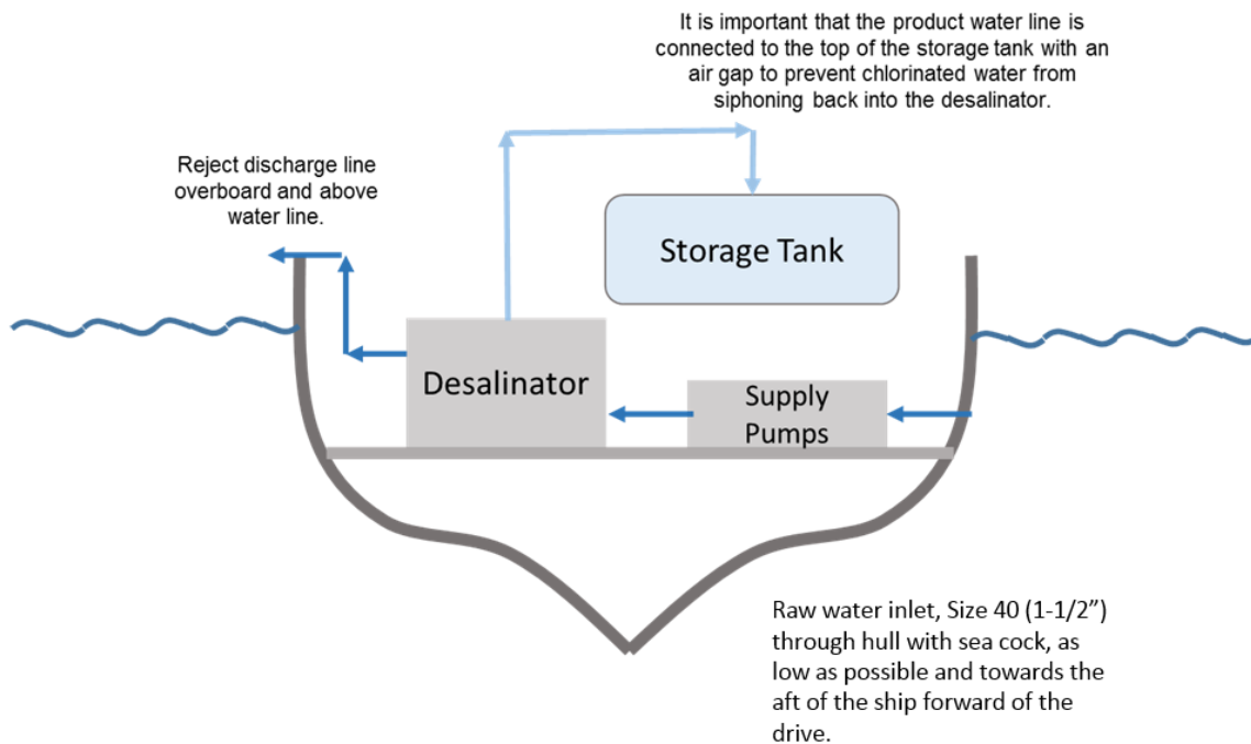
Figure 2.1 – RO Below Water Line
