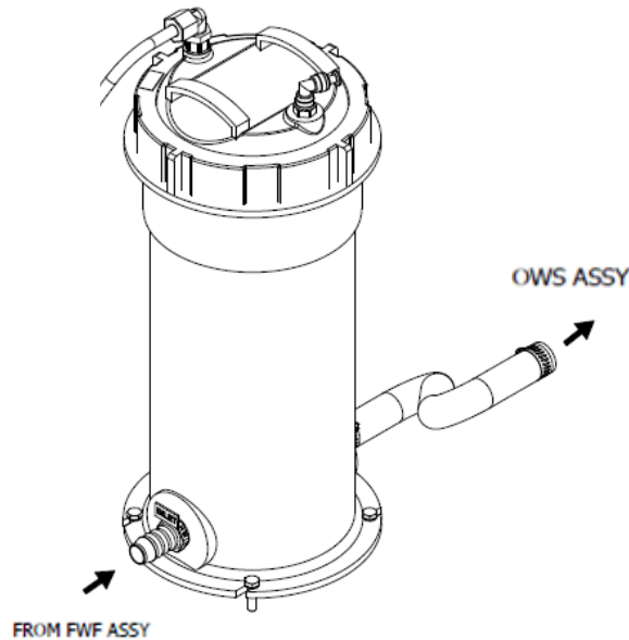
Figure 2.19: 5-Micron Prefilter Assembly
