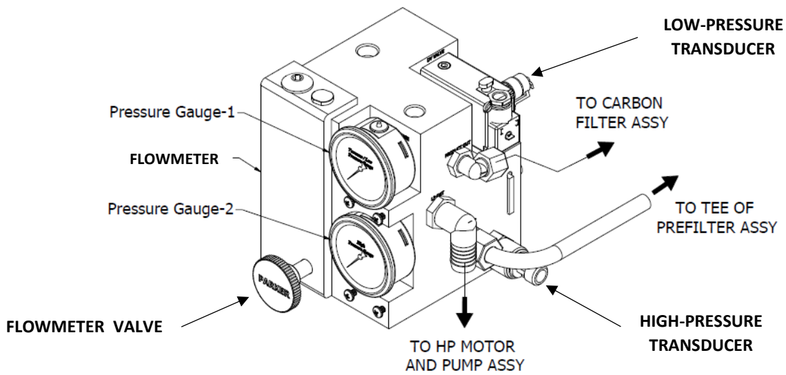
Figure 2.23: Manifold Assembly
