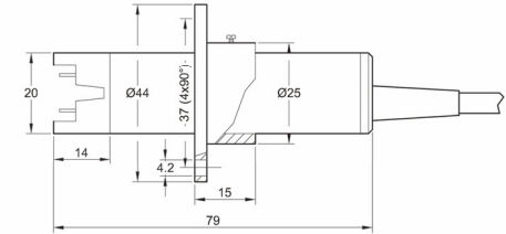
Type 3202.0x with flange
